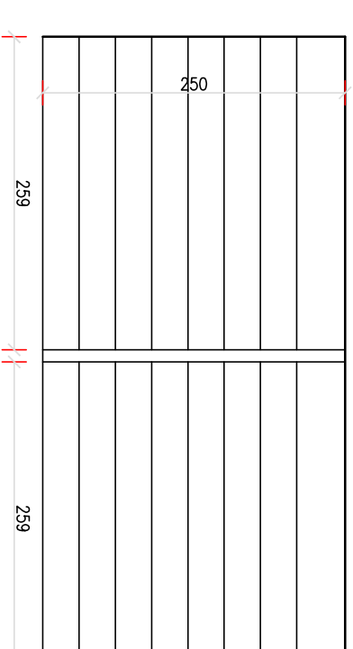
BRAMA GARAZOWA 2x - 260x250
